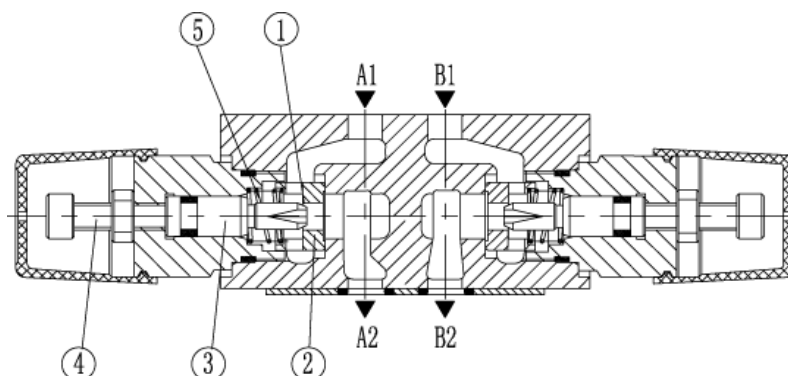
Type Z2FS6-2-40B/...
