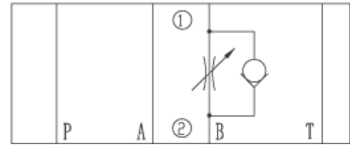
Z2FS 6B-...-40B/...(meter-in)
